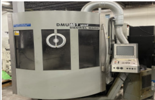
2004 DMG Deckel Maho Model 60T 5 Axis Machining Center, Heidenhain Mill Plus IT CNC Control
